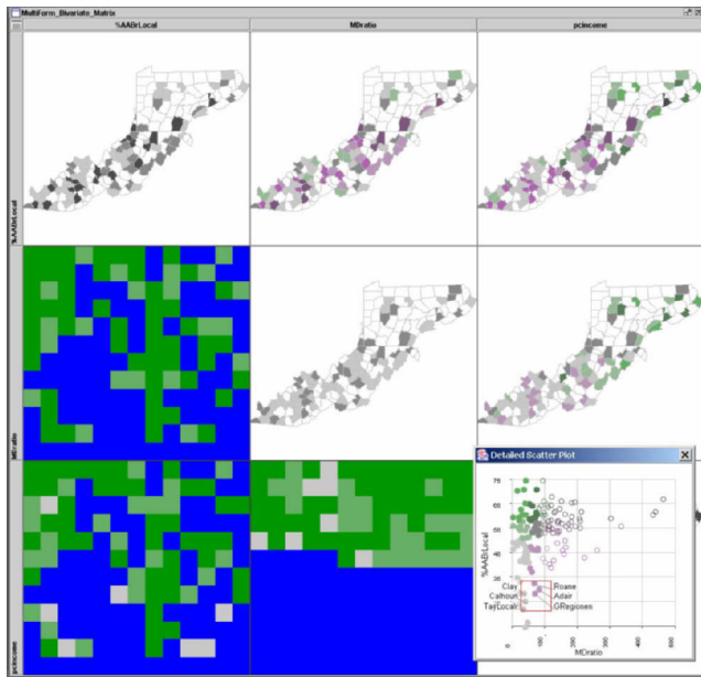
Figure 6. Matrix with bivariate map and spacefill components (univariate maps along the diagonal). Counties with a doctor ratio under about 80/1000 are highlighted in the popup scatterplot – with highlighting propagated to other views.
