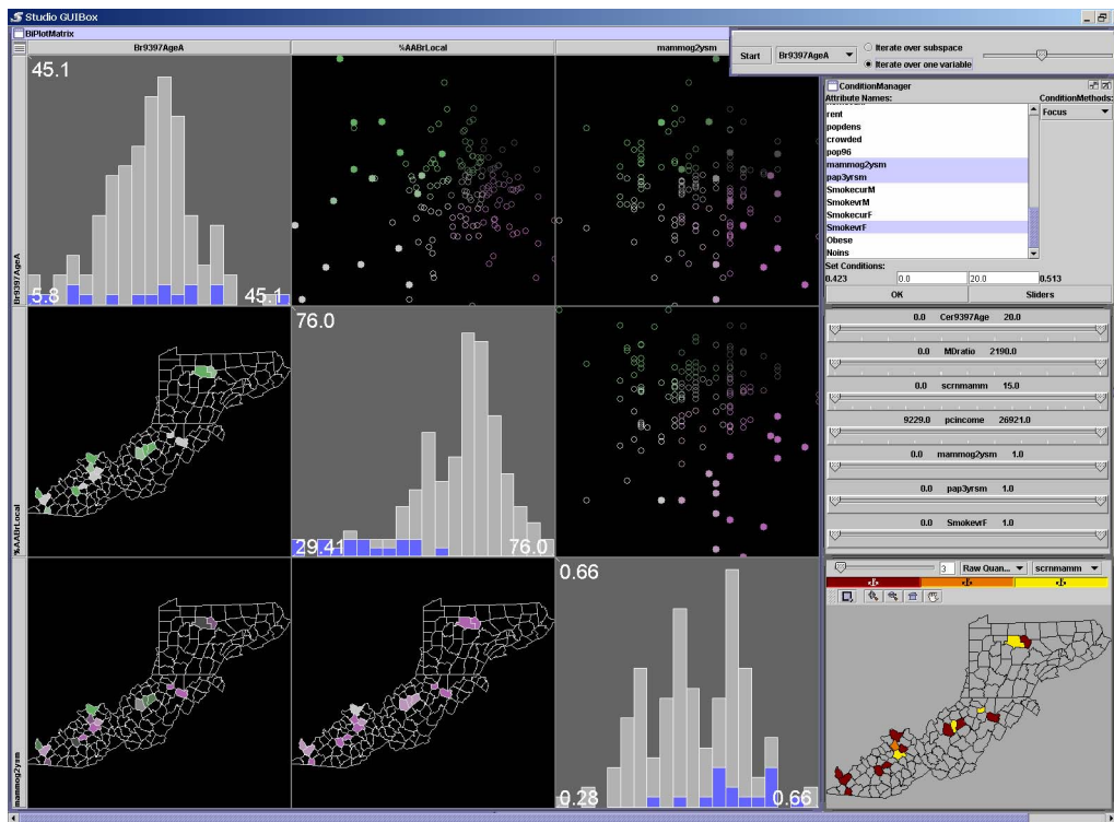
Figure 4. Typical display. MultiForm Bivariate Matrix with map and scatterplot (left), univariate map (lower right), conditioning picker and sliders generated by user selection (middle right), and conditioning animator (top right). An additive selection has been made in lower right scatterplot.
