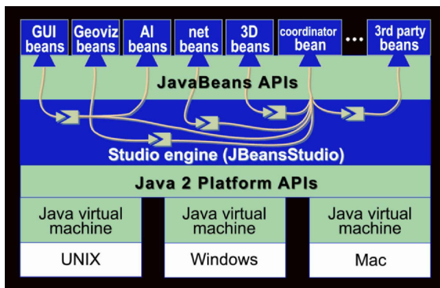
Figure 1. GeoVISTA Studio component-based architecture.
