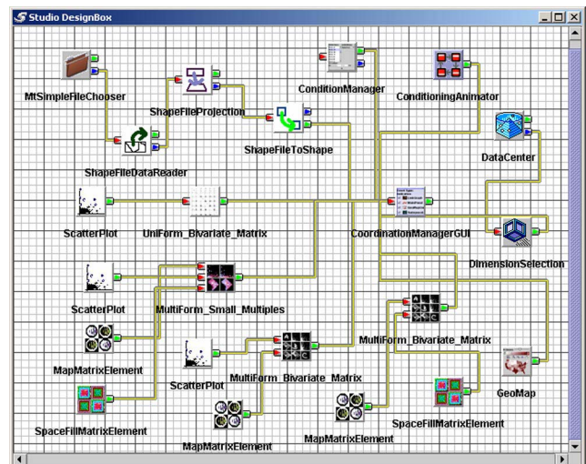
Figure 2. GeoVISTA Studio application design.
